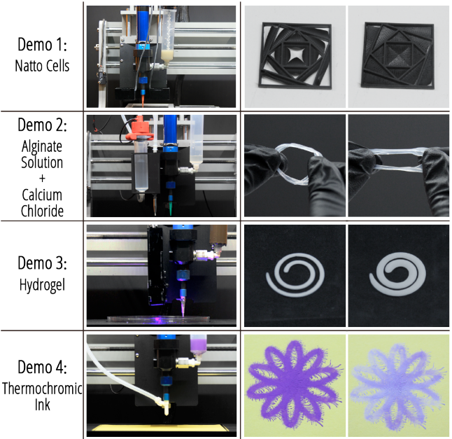
Figure 11: Four different modular configurations are used to print four different functional materials. Demo 1: Natto cells form humidity responsive films; Demo 2: Calcium alginate gels are stretchy and responsive to PH; Demo 3: UV-curable hydrogels swell in water; Demo 4: Thermo-chromic ink printed on paper.
