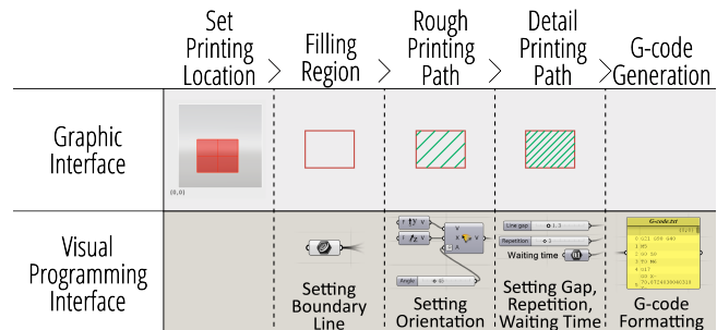
Figure 7: Graphic user interface for filling a 2D geometry.
